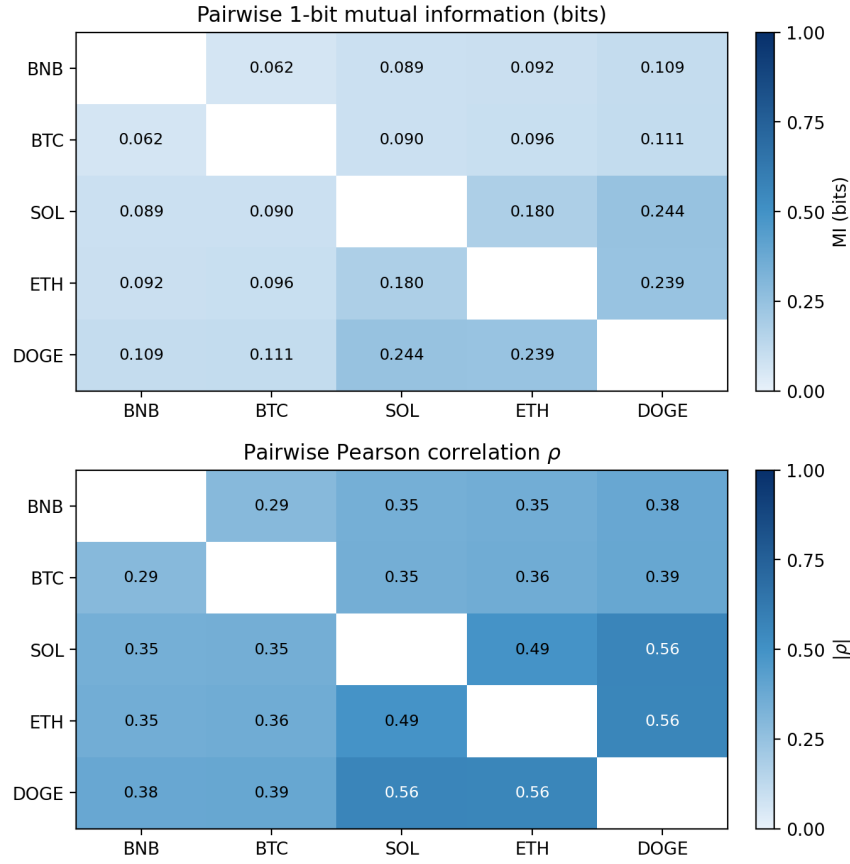
Figure 4.10: Experiment 4 – calibration-window mutual information matrix.
